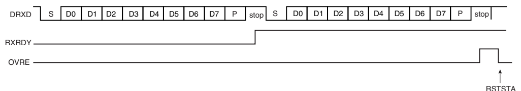
Figure 30-7. Receiver Overrun
